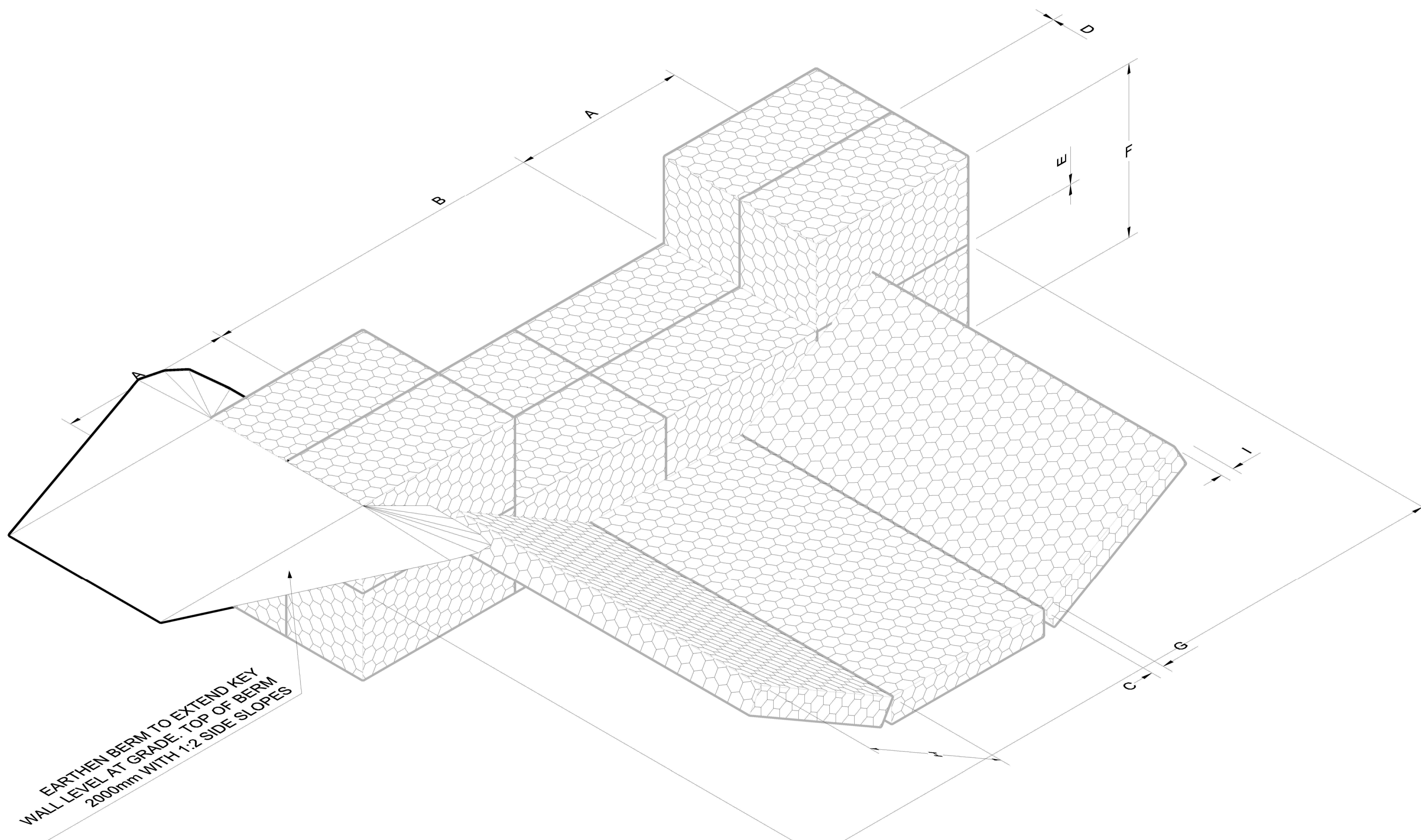
GABION PLUG ISOMETRIC VIEW SCALE 1:20
